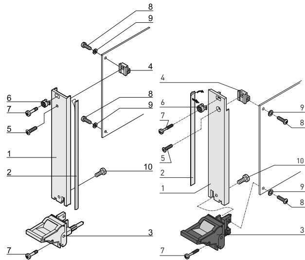
3 HE Fronteinbau
