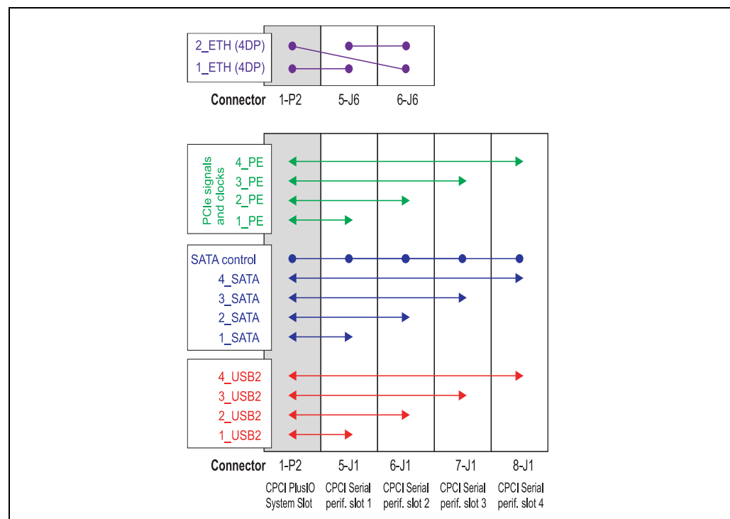
Figure 3: Backplane serial link routing
