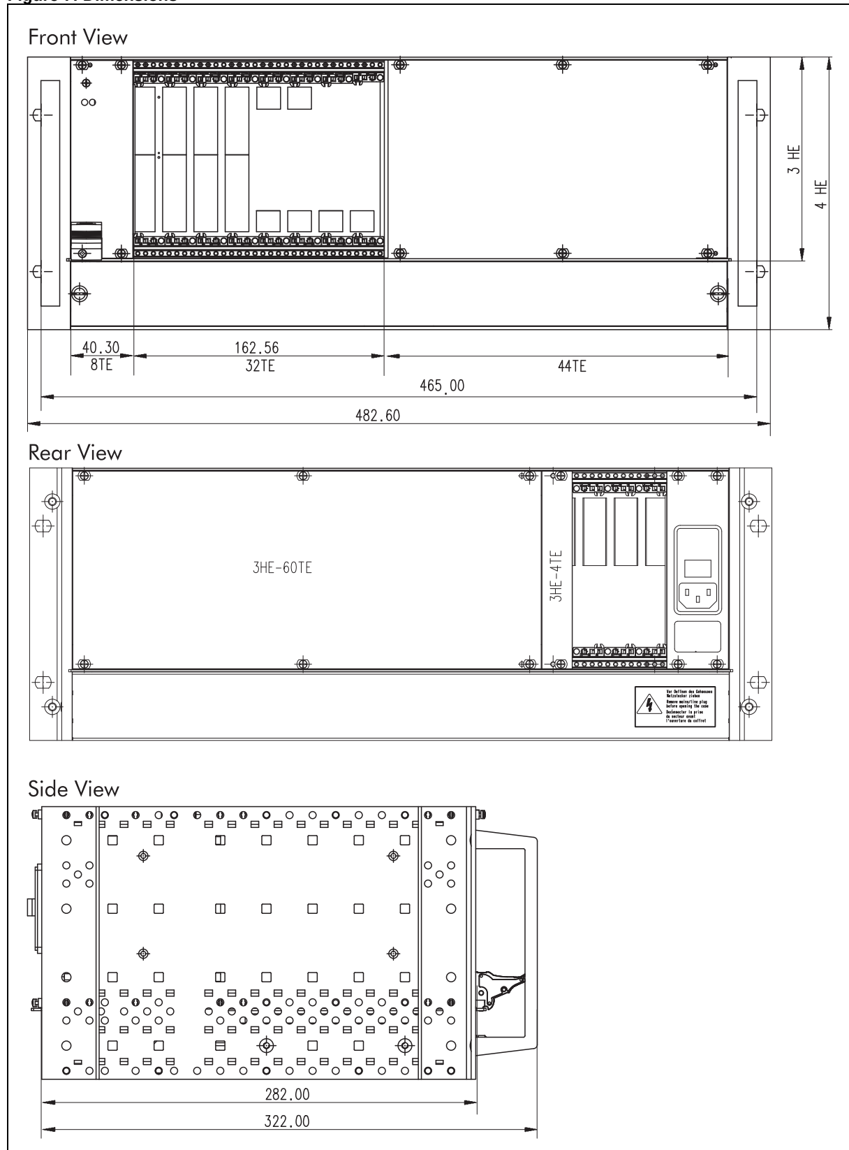
Figure 7: Dimensions
