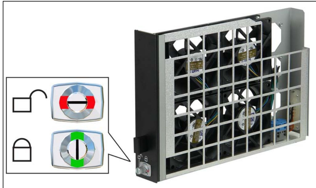
Figure 4: Fan Tray
