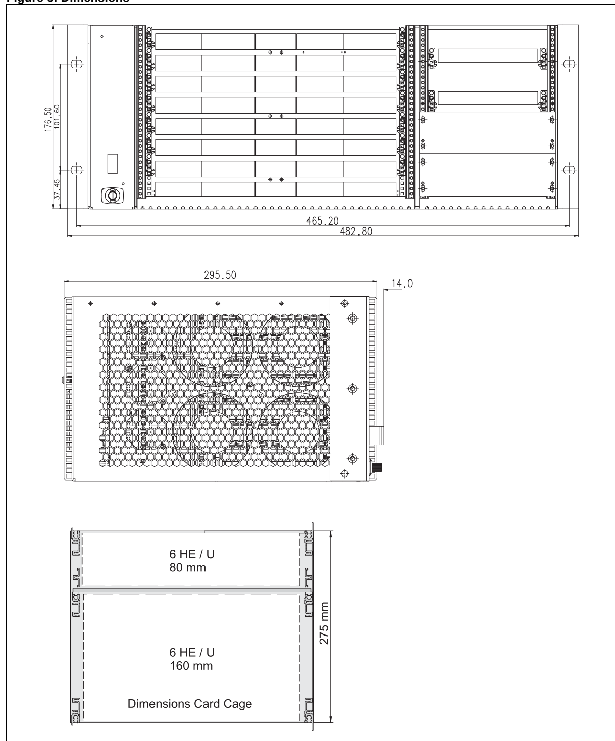
Figure 6: Dimensions
