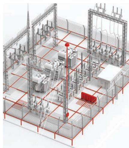
nVent ERICO System 3000 Collection Volume Method (Active System)
