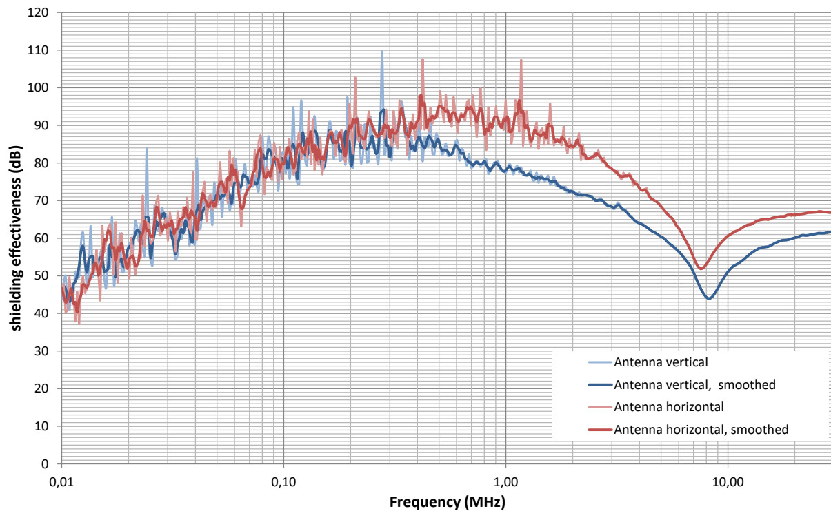
Shielding effectiveness 10 kHz - 30 MHz, Top
