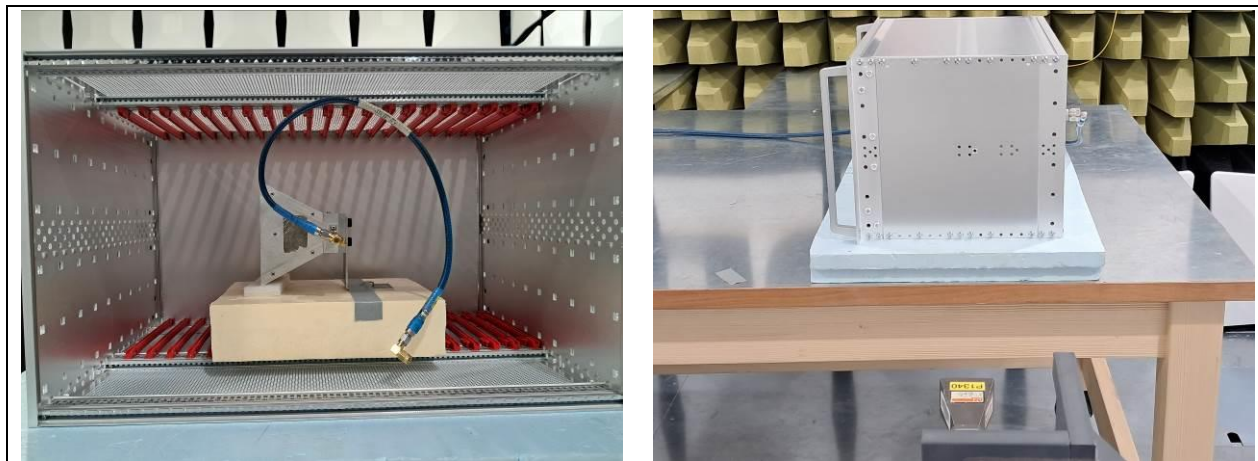
Figure 6-18: test setup horizontal, 18 – 40 GHz
