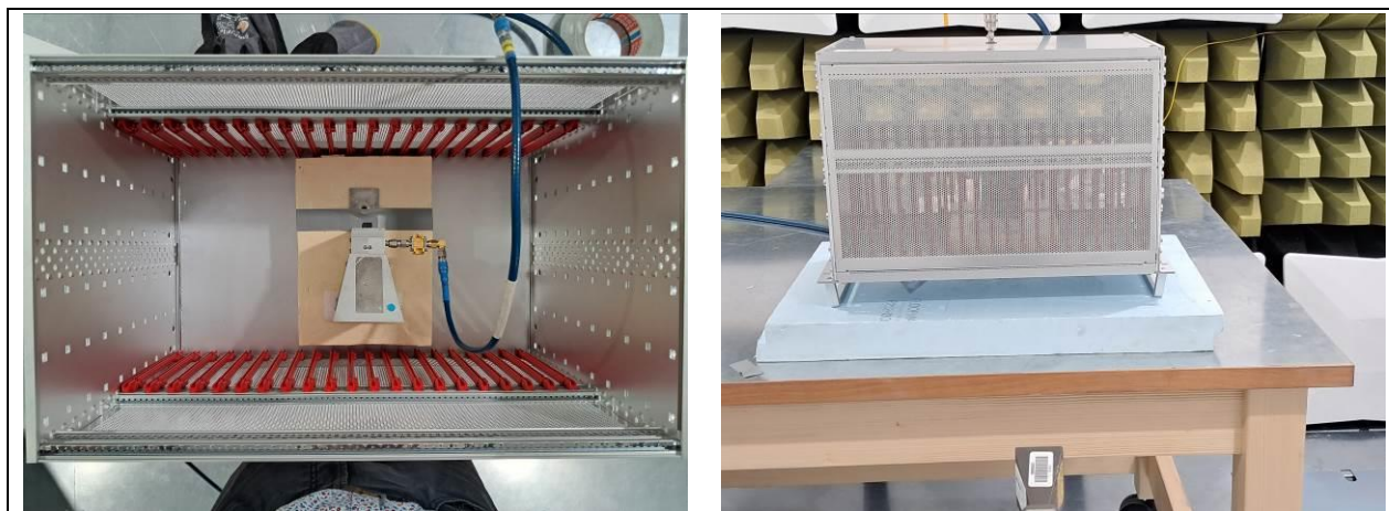
Figure 6-20: test setup horizontal, 18 – 40 GHz
