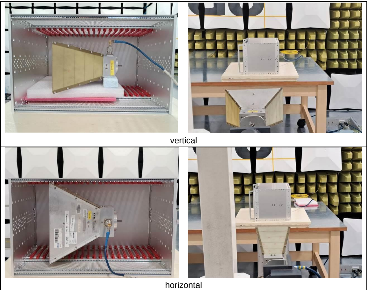
Figure 6-13: test setup 1 – 18 GHz
