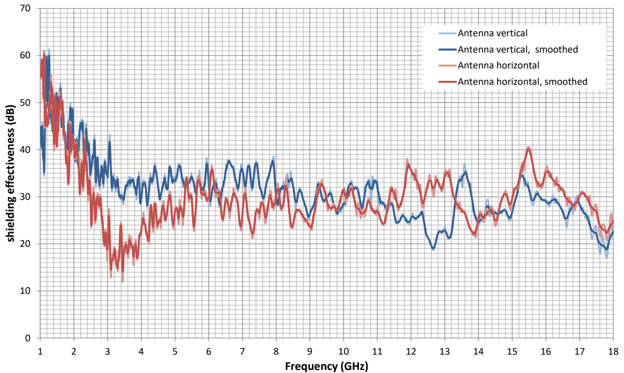
Shielding effectiveness 1 - 18 GHz, Top
